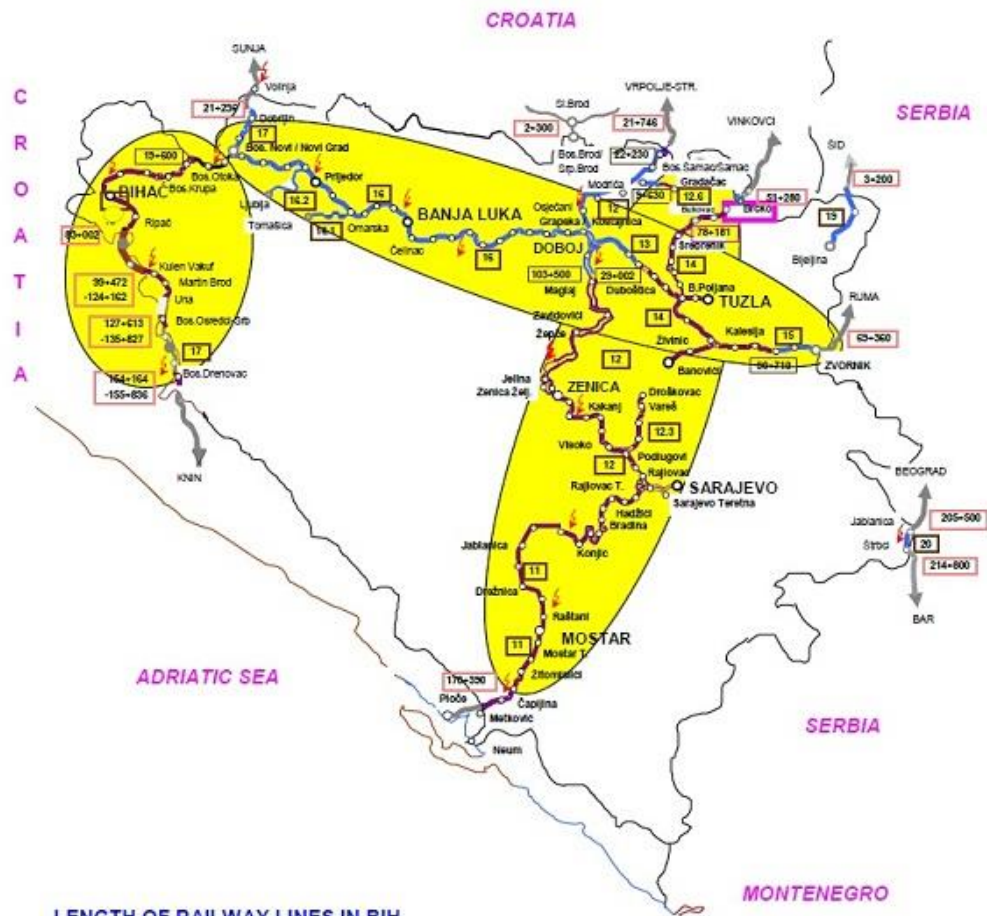
M A P OF RAILWAY SECTIONS TO BE COVERED WITH RECONSTRUCTION OF ELECTRO-ENERGETIC FACILITIES
